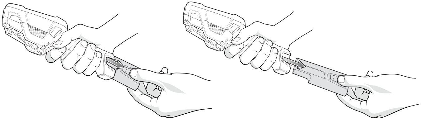
Figure 1-16 Battery Removal
