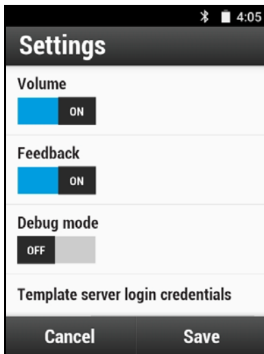
Figure 4-30 Settings Screen
