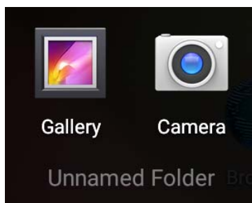
Figure 2-5 Open Folder
