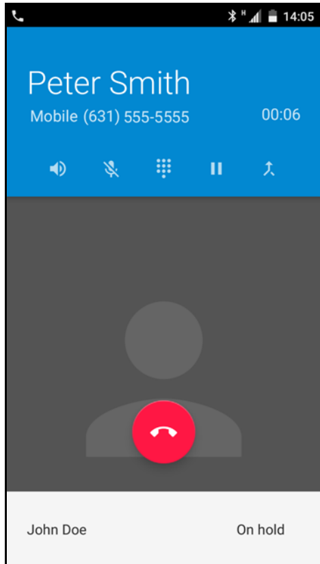
Figure 3-8 Two Calls
