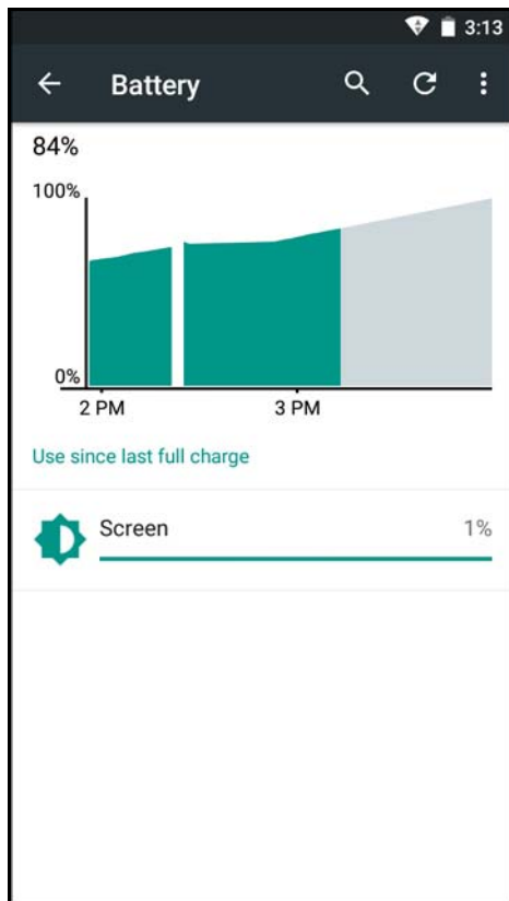
Figure 1-29 Battery Screen
