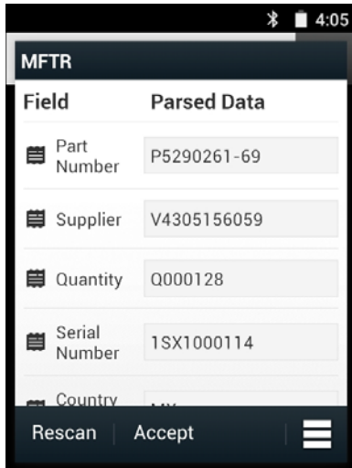
Figure 4-29 Manufacturing Data
