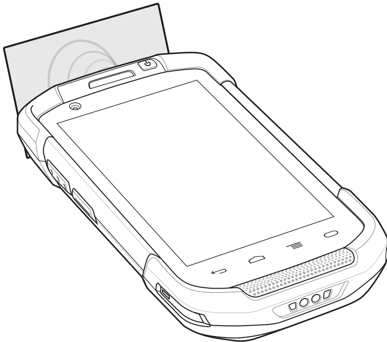
Figure 6-14 Reading Cards
