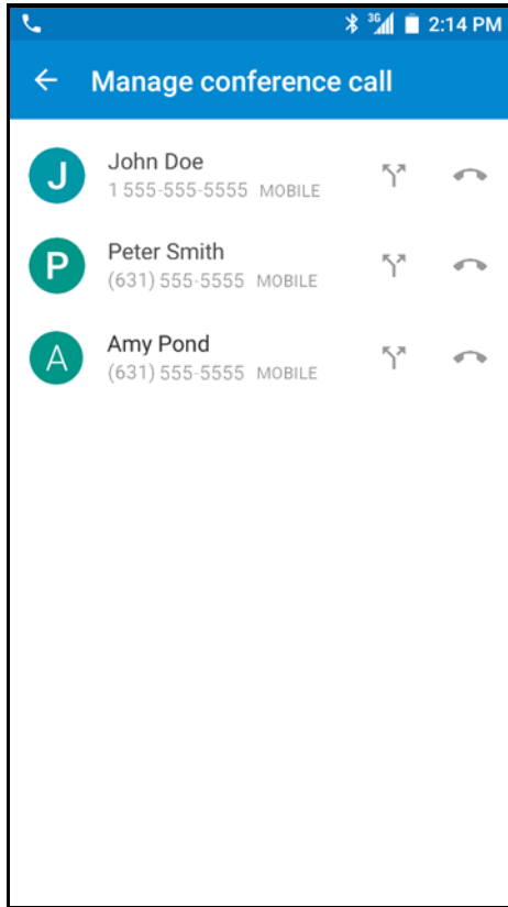
Figure 3-10 Un-merge Calls
