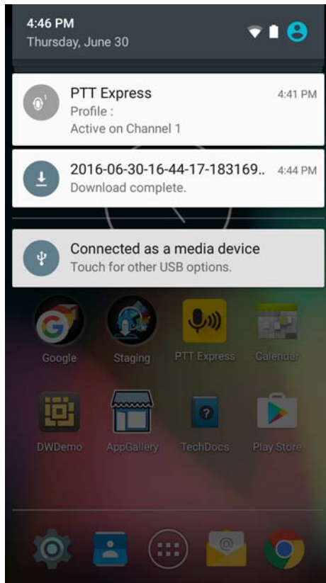
Figure 2-3 Notification Panel
