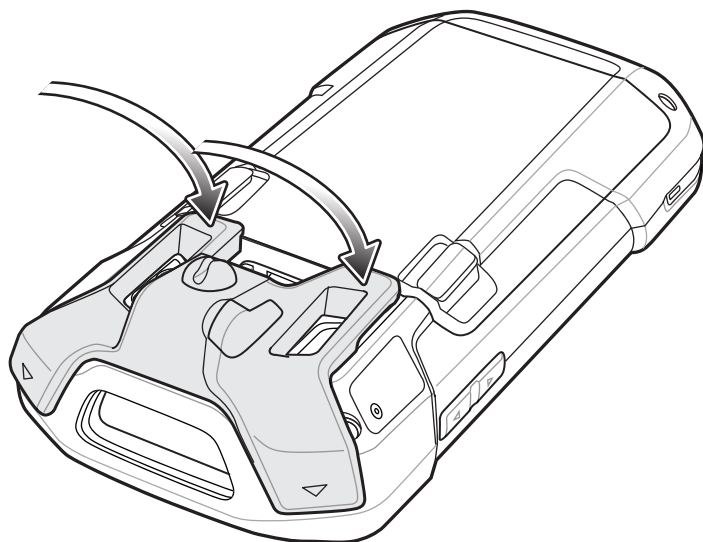
Figure 119: Rotate Audio Adapter onto TC70
