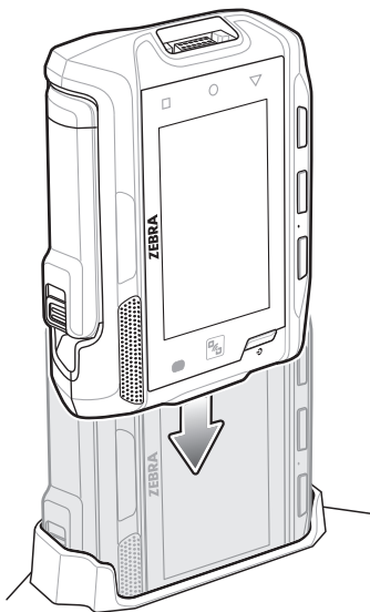
Figure 43 Insert WT6000 into Cradle
