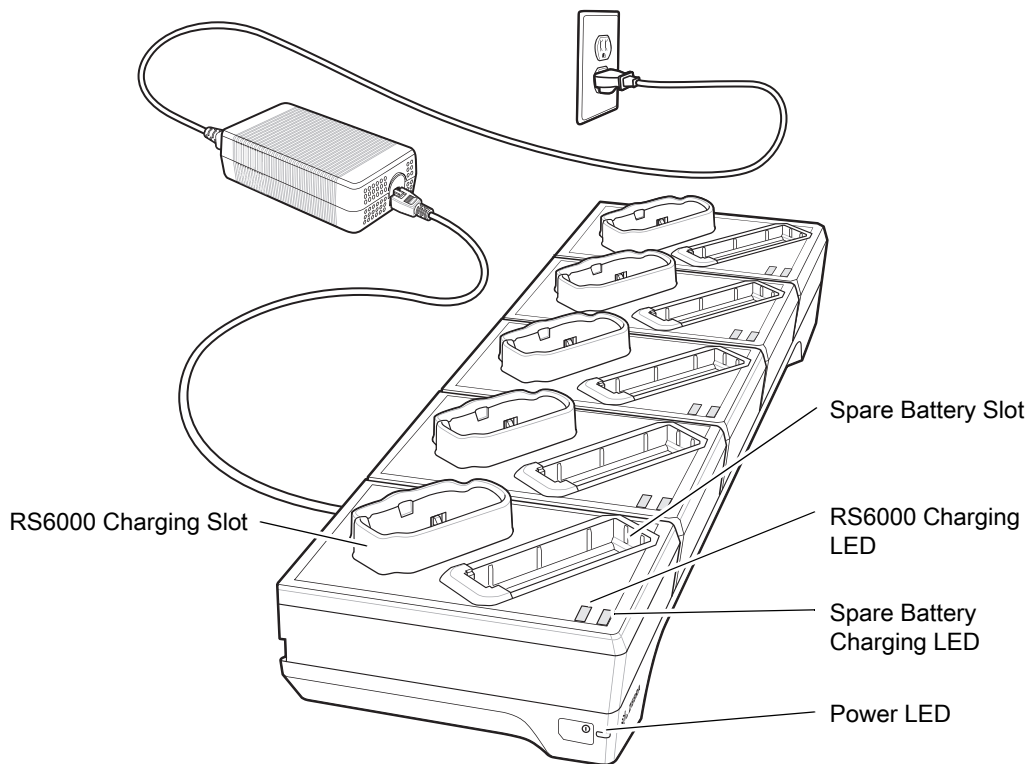
Figure 37 5-Slot RS6000 Charge Only Cradle
