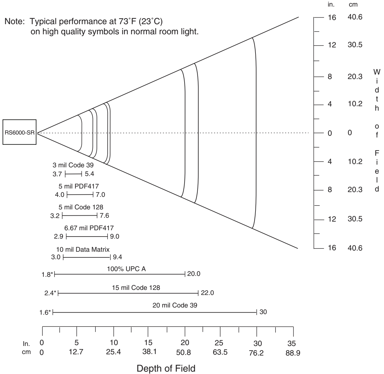
Figure 83 RS6000 Standard Range Decode Zone
