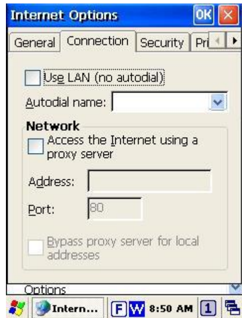
Figure 8-11-2 Internet Options
