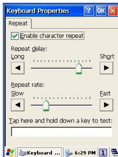
Figure 8-12 Keyboard Properties
