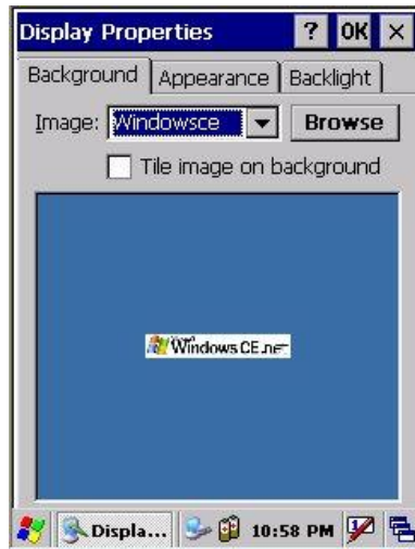
Figure 8-9-1 Display Properties
