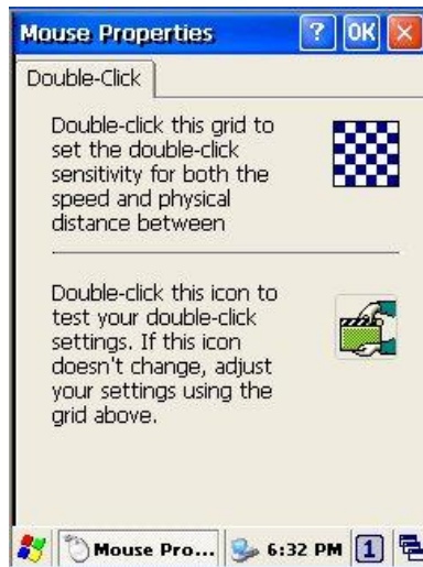
Figure 8-13 Mouse Properties
