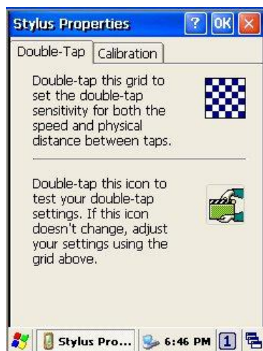
Figure 8-21 Stylus Properties
