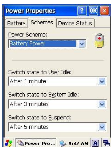
Figure 3-8 Power Properties
