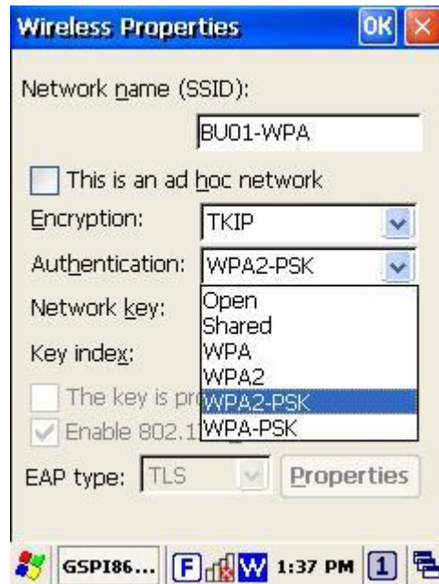
Figure 3-31 Wireless Properties
