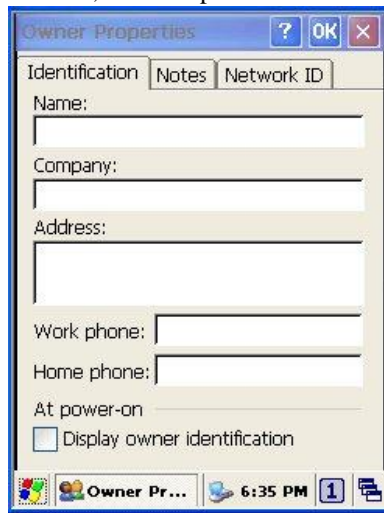
Figure 8-15 Owner Properties
