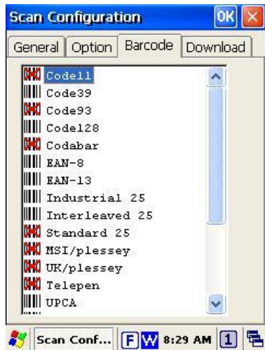
Figure 4-1-3 Scan Configuration
