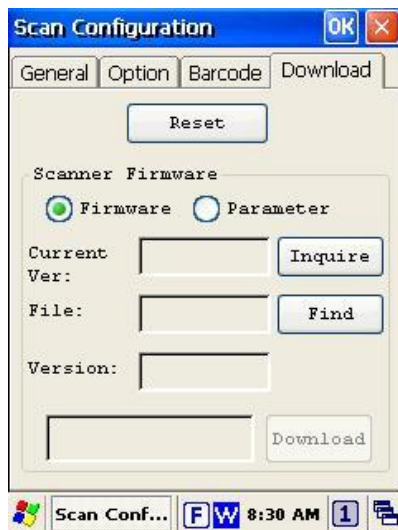
Figure 4-1 -4 Scan Configuration
