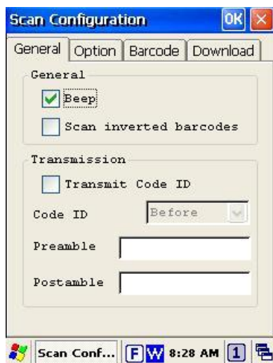
Figure 4-1-2 Scan Configuration
