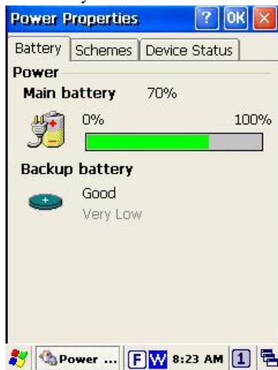
Figure 3-7 Power Properties
