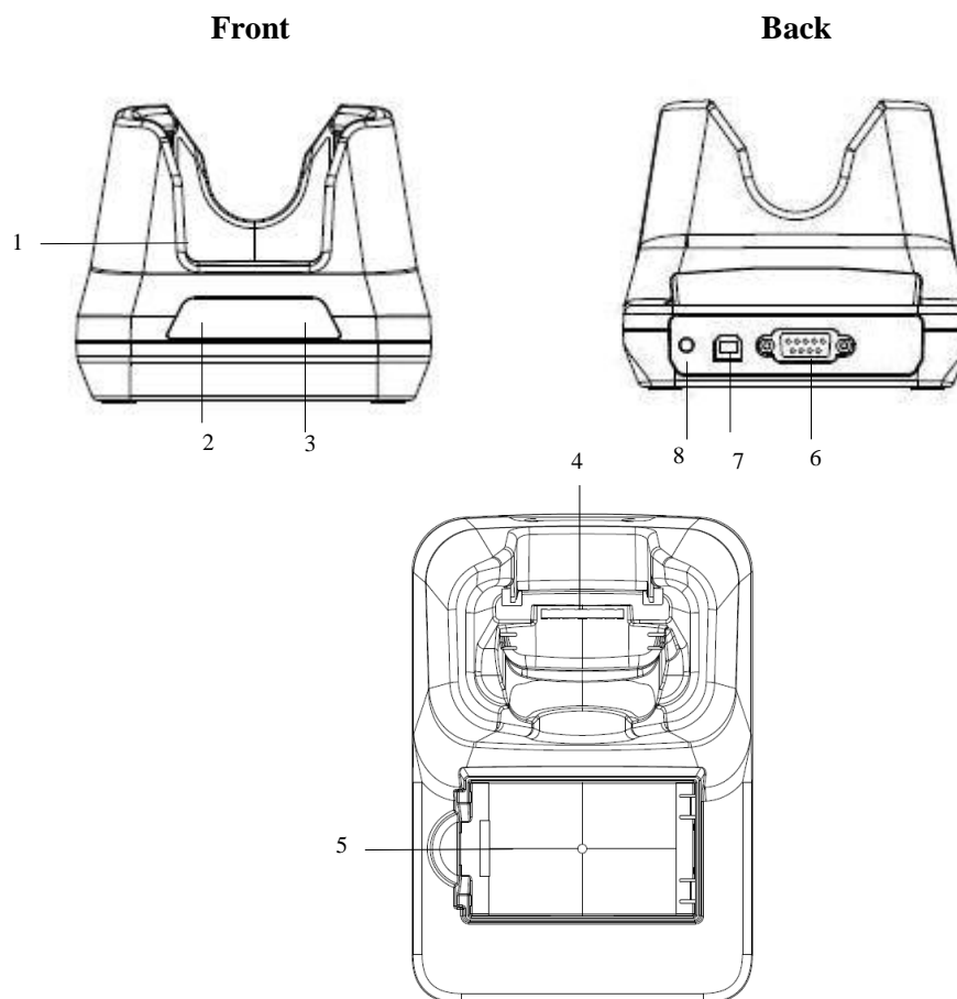
Figure 2-4 The Details of Cradle
