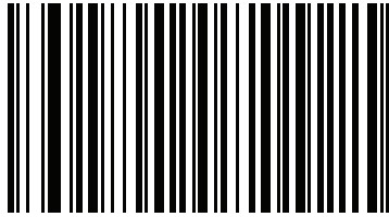
Chinese 2 of 5
