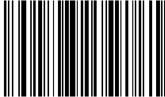
15 Characters
