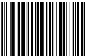
Send Q
