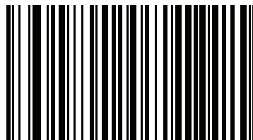
Matrix 2 of 5
