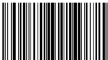
Send K
