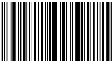
Send Control 6
