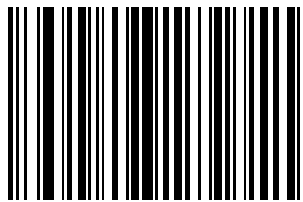
Send W
