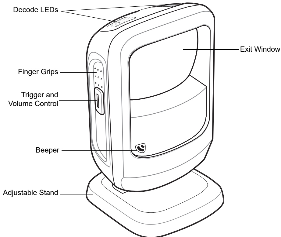
Figure 2-1 Parts
