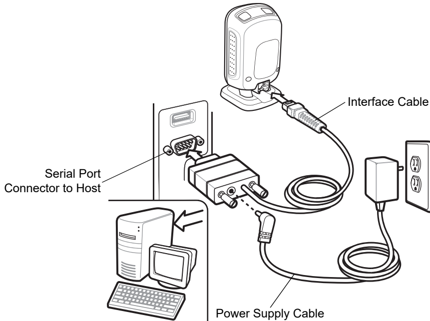
Figure 6-1 RS-232 Direct Connection
