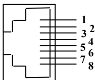
8-pin
